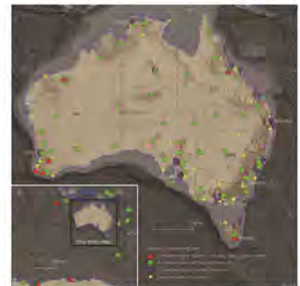
Image courtesy of Geoscience Australia. Map showing location of Seismic Monitoring Stations around Australia
